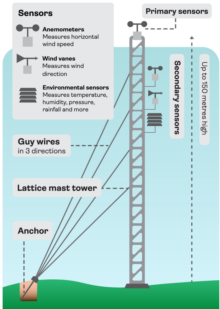
Figure 3: Meteorological mast diagram. Artist's impression only, not to scale.
